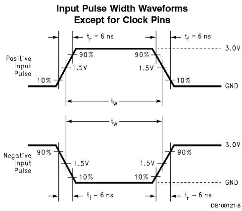
FIGURE 4. Switching Characteristic Measurement Waveforms
